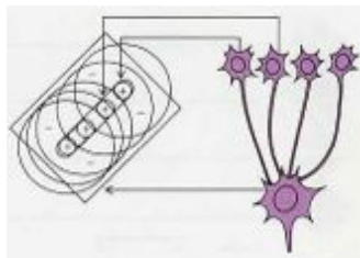
Figure 1: Hubel and Wiesel's scenario for the transition between the receptive profiles in the LGN and those in V1: if the electrical activity of a neuron in V1 is close to the sum of activities exhibited by LGN cells which have the centers of their receptive profiles distributed on a small segment of the visual plane, the cortical neuron will have a clear orientation preference.
