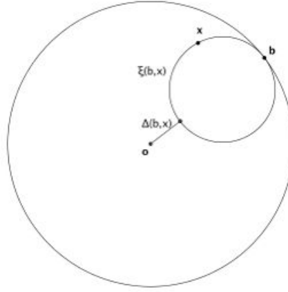
Figure 3: A horocycle in \mathbb{D} .
