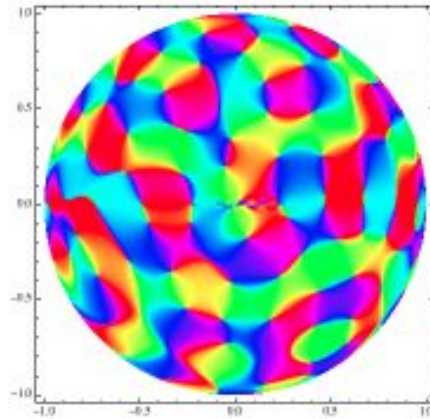
Figure 7: An orientation map on the sphere sampled from a random vector field which has SO(3) -shift-twist symmetry. We plotted the restriction to a hemisphere of the random map exploring \mathcal{H}_{10}^{exact} ; beware that the color coding has a different meaning than in Figs. 1, 2, 5, 6. Here, the sample map is a vector field on the sphere, and there is no complex number; to visualize the direction of the emerging vector at each point, we apply the orthogonal projection from the drawn hemisphere to the "paper" plane, thus getting a vector field on the unit ball of the Euclidean plane, and plot the resulting orientation map using the same color code as in Fig. 1, 2, 5, 6.
