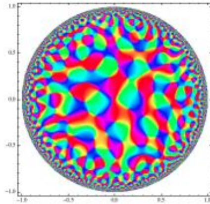
Figure 5: Plot of a monochromatic “orientation map” on the hyperbolic plane. We used the spectral parameter \omega = 18 in units of the disk’s radius. Because of the growth factor in the modulus of the e_{\omega,b} , drawing a picture in which discretization effects do not appear calls for using more propagation directions than it did in the Euclidean case: 200 directions were used to generate the drawn picture.
